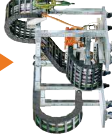
Prototype including transport rack
